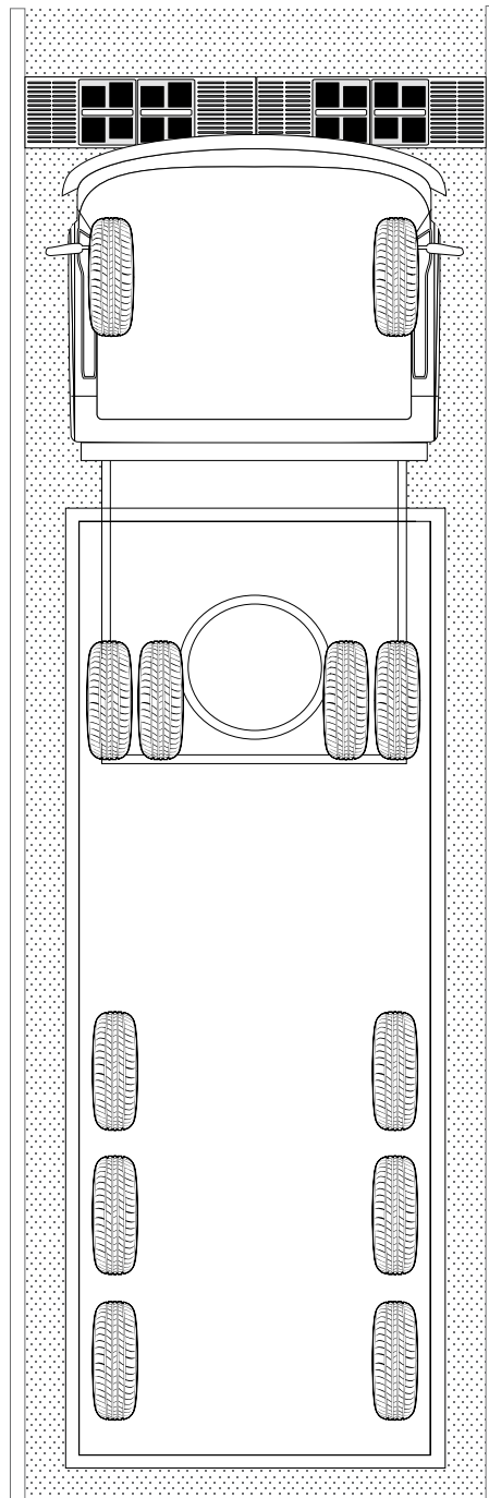
Schematic drive-over situation of a five-axle articulated lorry.
